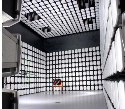
10 m Semi-Anechoic Room
